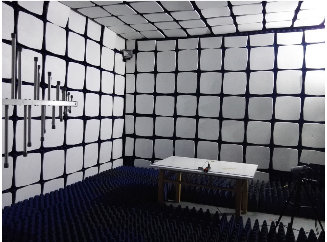
14.5 Photo of RF Field Strength susceptibility Test
